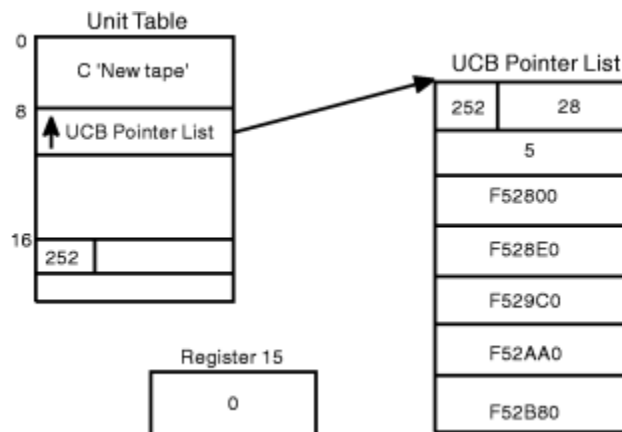
Figure 118. Output from Function Codes 3 and 10
