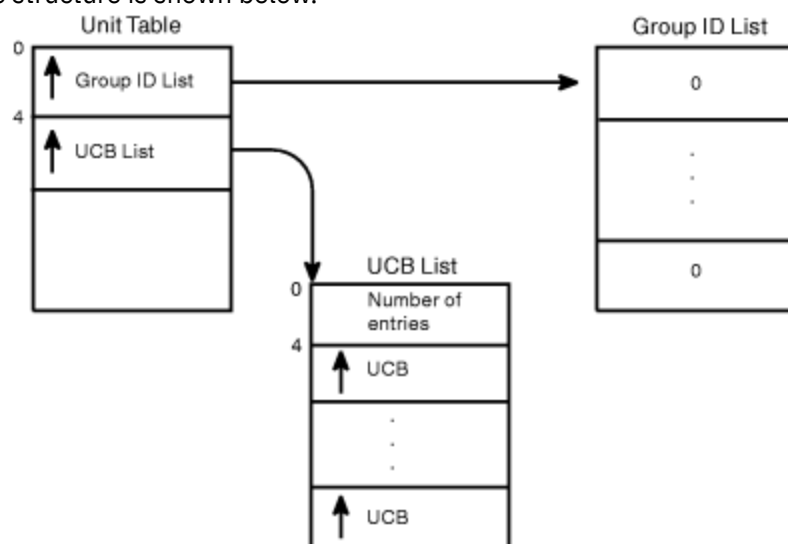
Figure 104. Requesting Function Code 4 (Return Group ID)
