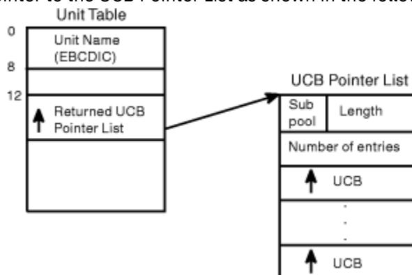
Figure 103. Output from Function Code 3 (Return UCB Addresses)
