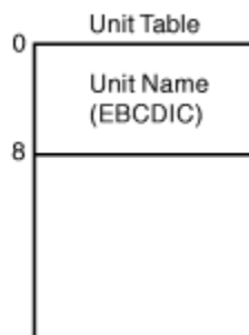
Figure 101. Output from Function Code 2 (Return Unit Name)
