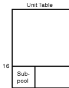
Figure 112. Requesting Function Code 10 (Specify Subpool for Returned Storage)
