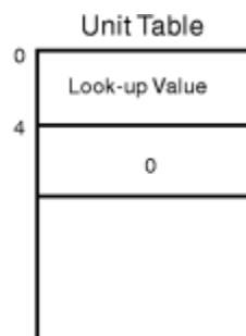
Figure 106. Requesting Function Code 5 (Indicate Unit Name is a Look-up Value)
