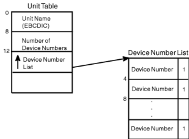
Figure 99. Requesting Function Code 1 (Check Units)
