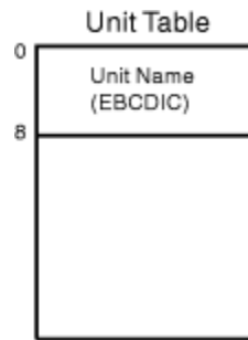
Figure 107. Requesting Function Code 6 (Return Look-up Value)
