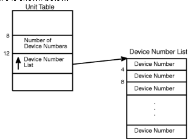
Figure 98. Requesting Function Code 0 (Check Groups)
