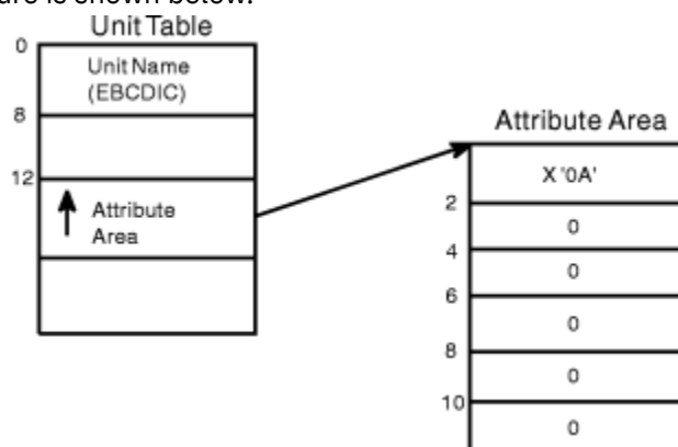
Figure 111. Requesting Function Code 8 (Return Attributes)
