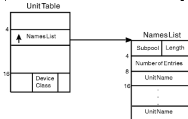
Figure 114. Output from Function Code 11 (Return Unit Names for a Device Class)
