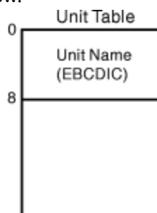
Figure 102. Requesting Function Code 3 (Return UCB Addresses)
