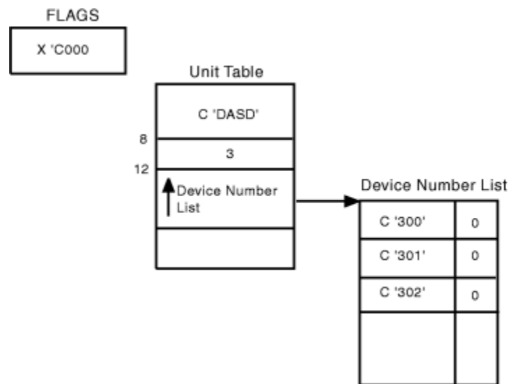
Figure 115. Input for Function Codes 0 and 1
