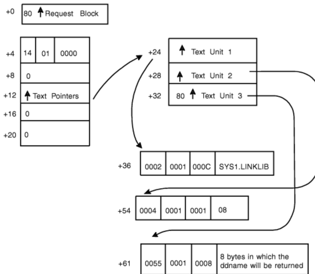
Figure 70. Parameter List Resulting from Dynamic Allocation Example
