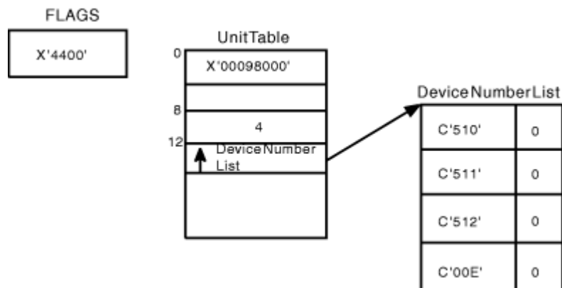
Figure 119. Input for Function Codes 1 and 5
